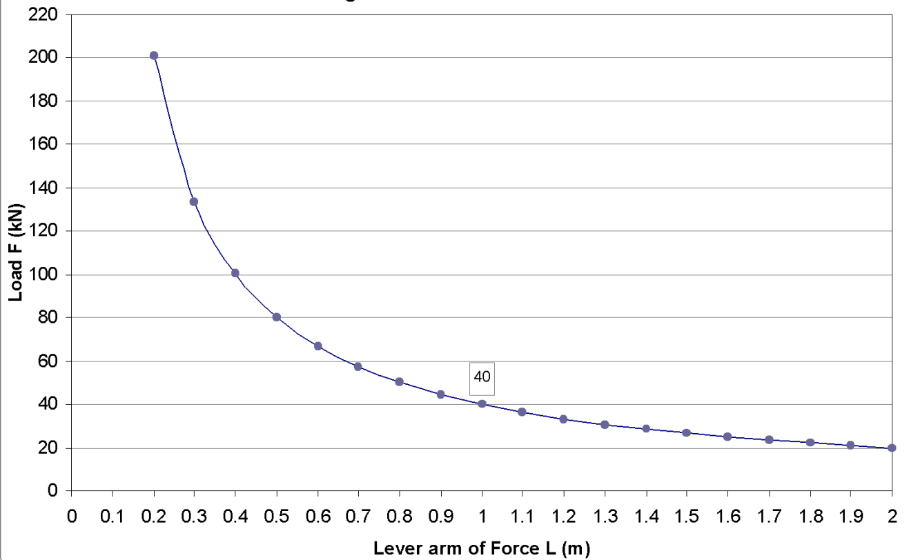
Load diagram for rotator CPR 15 series
